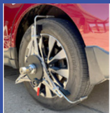
3-Point Touchless Wheel Clamp Adapters ...No Rolling of the Vehicle
